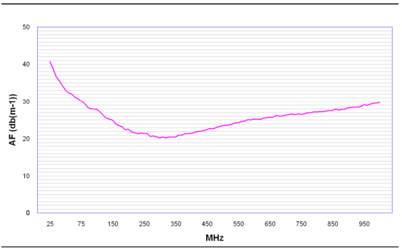
Antenna factor BicoLOG 20100 EX
