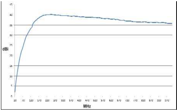
Gain Diagram BicoLOG 20100 EX
