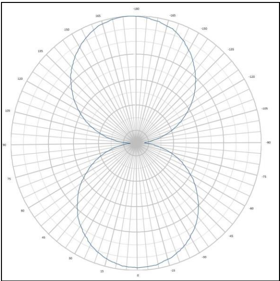
Horizontal Pattern (typical) BicoLOG Anten
