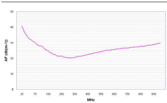
Antenna factor BicoLOG 20100 X
