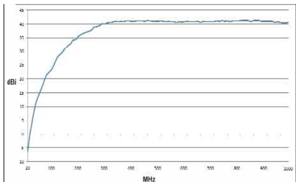
Gain Diagram BicoLOG 20100 X
