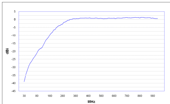
Gain Diagram BicoLOG 30100
