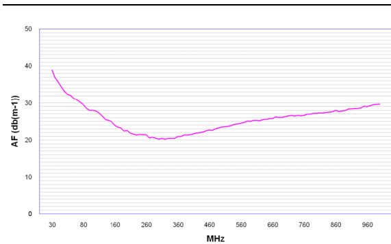
Antenna factor BicoLOG 30100
