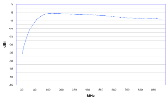
Gain Diagram BicoLOG 30100E
