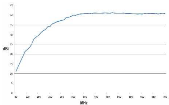
Gain Diagram BicoLOG 5070X
