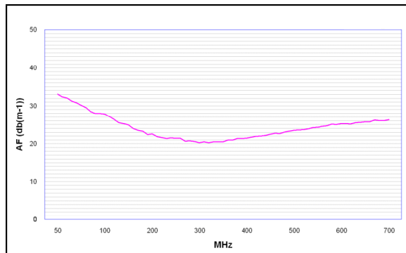
Antenna factor BicoLOG 5070X
