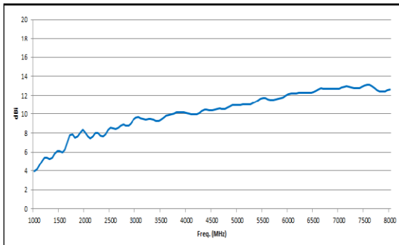
Gain PowerLOG 10800 Gain
