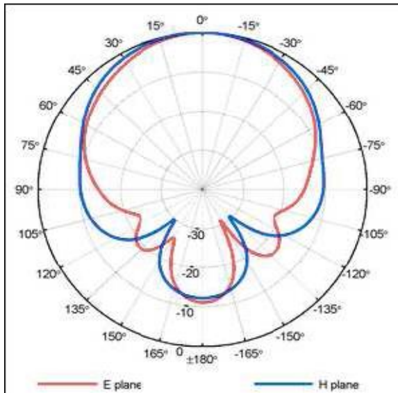
Typ. 1GHz Pattern
