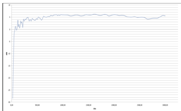
Gain Diagram HyperLOG 20300 EMI (10m)
