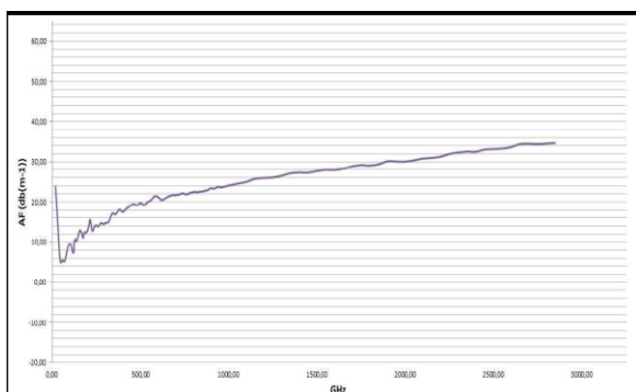
Antenna factor HyperLOG 20300 EMI
