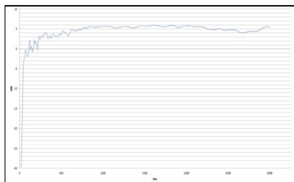
Gain Diagram HyperLOG 20300 EMI (3m)
