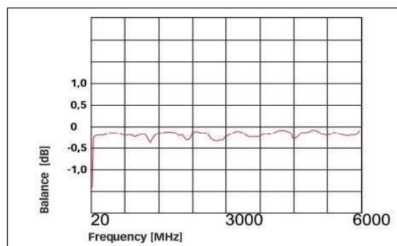
Typical Balance / Unbalance
