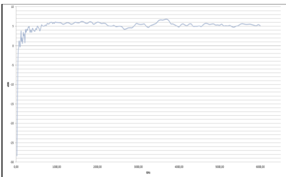
Gain Diagram HyperLOG 20600 EMI (10m)
