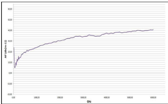
Antenna factor HyperLOG 20600 EMI
