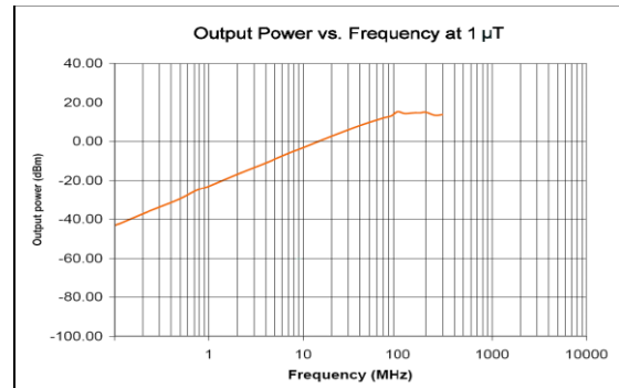
50mm magnetic field probe
