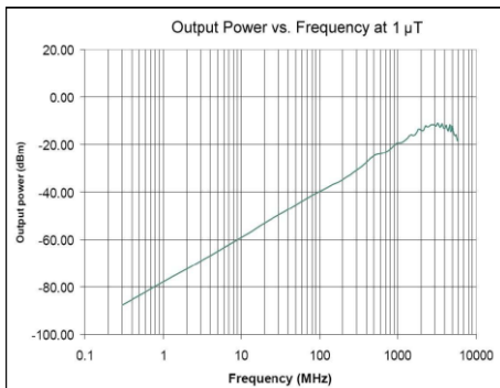
6mm magnetic field probe
