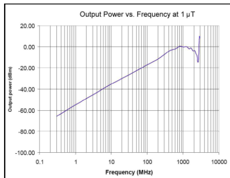
12mm magnetic field sniffer
