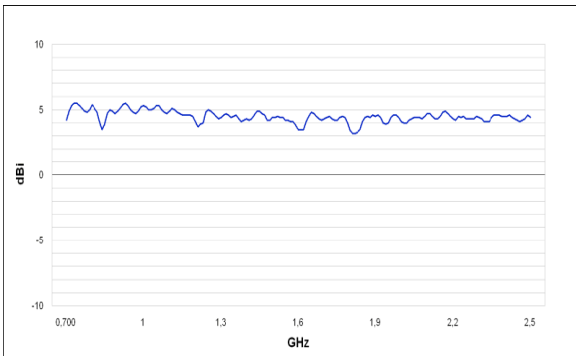
Gain Diagram HyperLOG 7025
