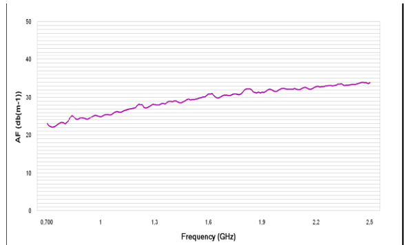
Antenna factor HyperLOG 7025
