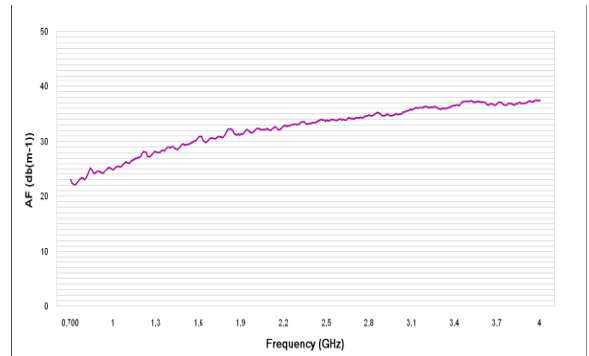
Antenna factor HyperLOG 6080
