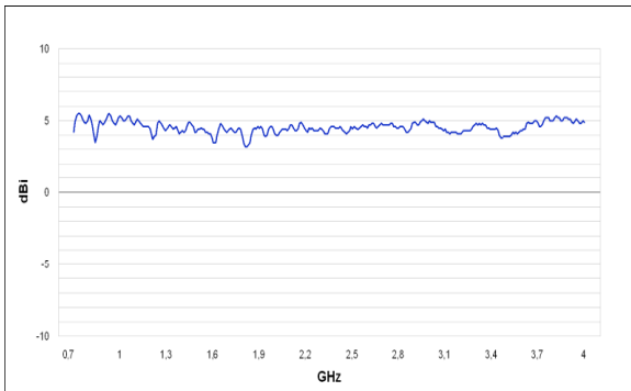
Gain Diagram HyperLOG 6080
