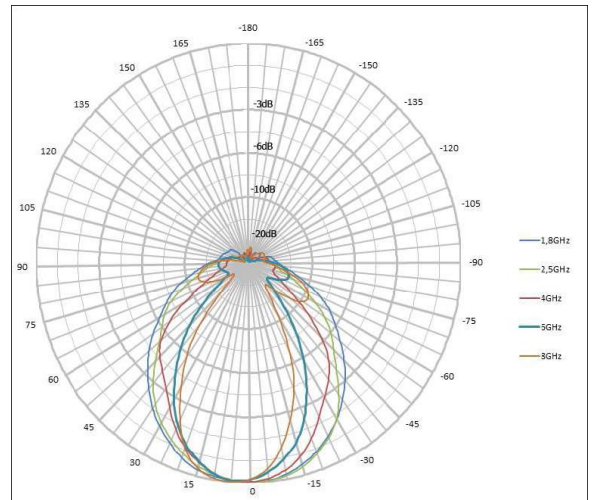
Vertical Pattern (typical) HyperLOG 60xx Series
