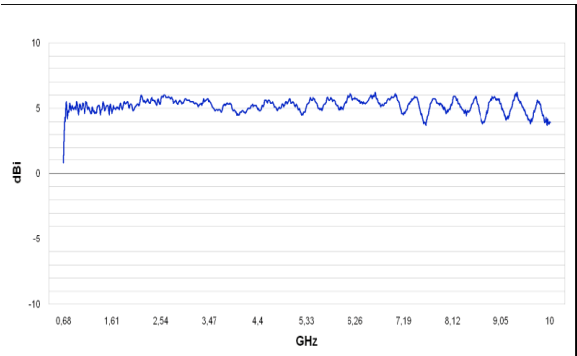
Gain Diagram HyperLOG 60100
