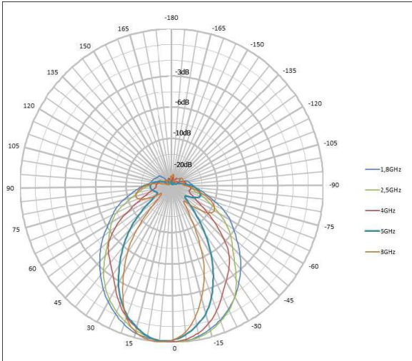
Vertical Pattern (typical) HyperLOG 60xx Series
