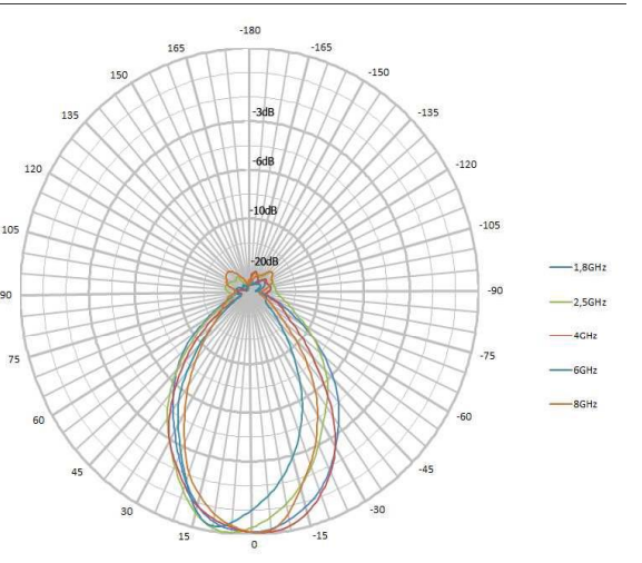
Horizontal Pattern (typical) HyperLOG 60xx Series
