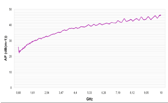
Antenna factor HyperLOG 60100
