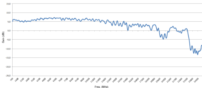
Gain Diagram HyperLOG 60250
