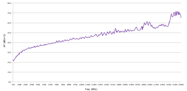
Antenna factor HyperLOG 60250
