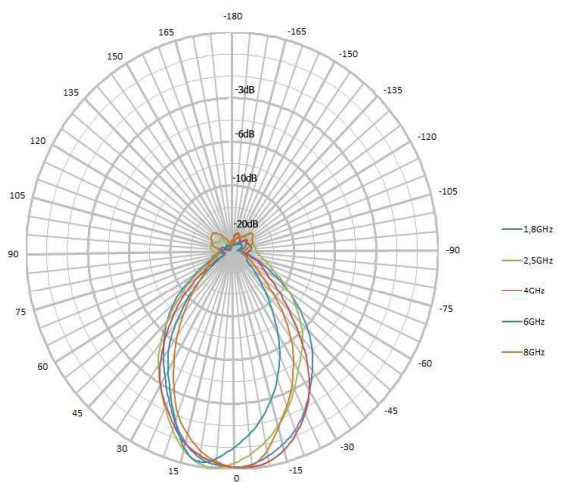
Horizontal Pattern (typical) HyperLOG 60xx Series
