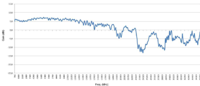
Gain Diagram HyperLOG 60350
