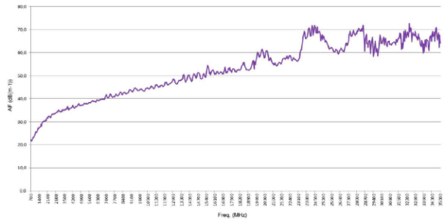
Antenna factor HyperLOG 60350
