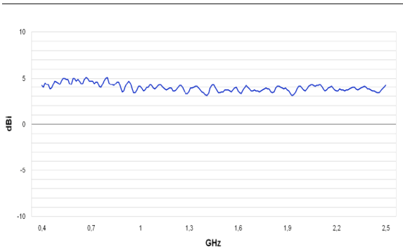
Gain Diagram HyperLOG 4025
