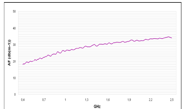
Antenna factor HyperLOG 4025
