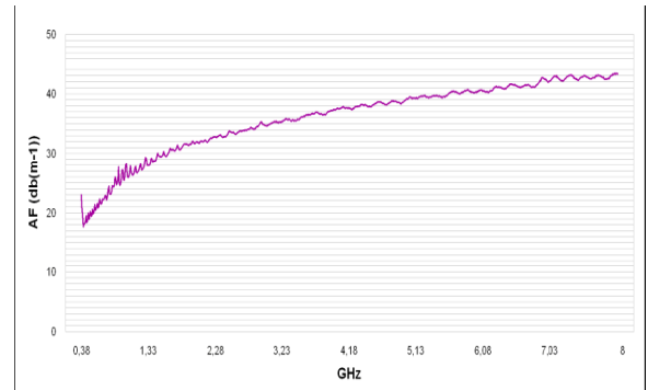
Antenna factor HyperLOG 3080
