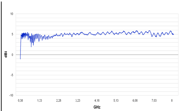
Gain Diagram HyperLOG3080
