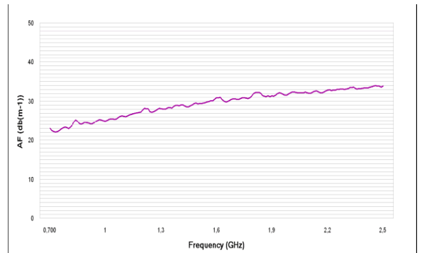
Antenna factor HyperLOG 7040 X
