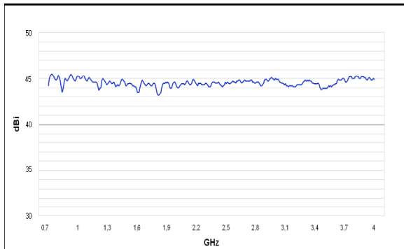
Gain Diagram HyperLOG 7040 X
