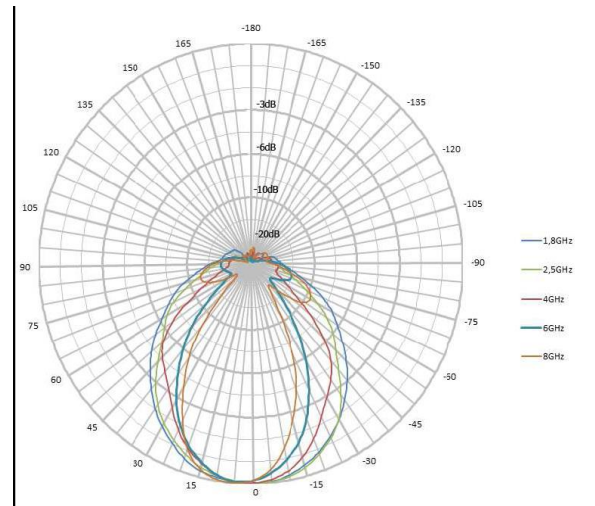
Vertical Pattern (typical) HyperLOG70x Series
