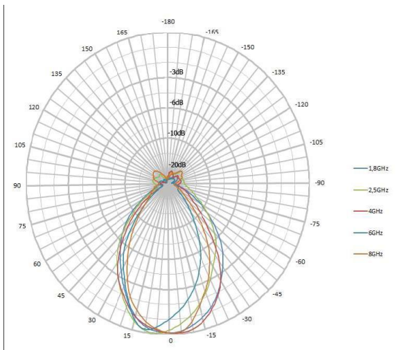
Horizontal Pattern (typical) HyperLOG 70x Series
