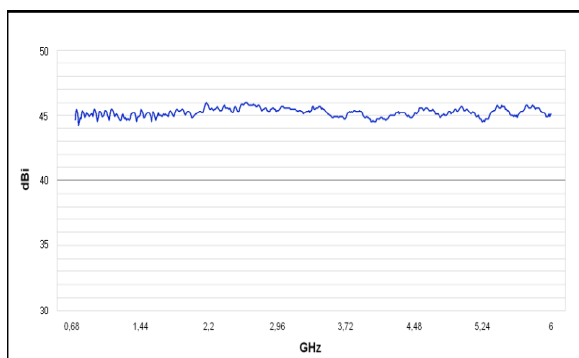
Gain Diagram HyperLOG 7060X
