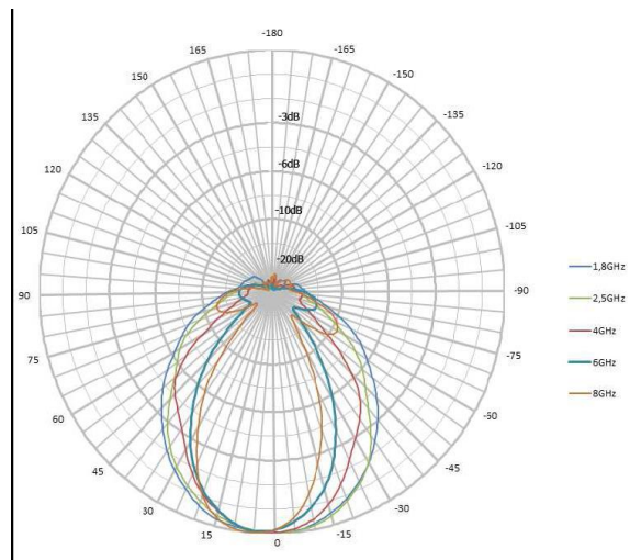
Vertical Pattern (typical) HyperLOG70x Series
