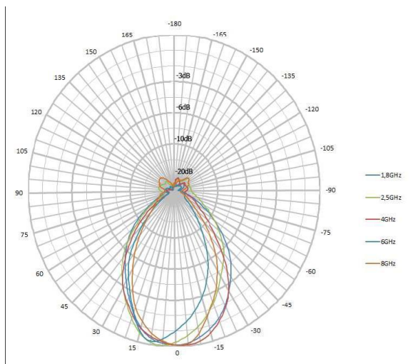
Horizontal Pattern (typical) HyperLOG 70x Series
