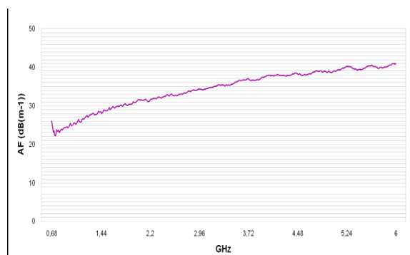
Antenna factor HyperLOG 7060X
