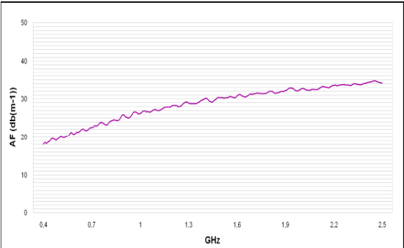
Antenna factor HyperLOG 4025 X
