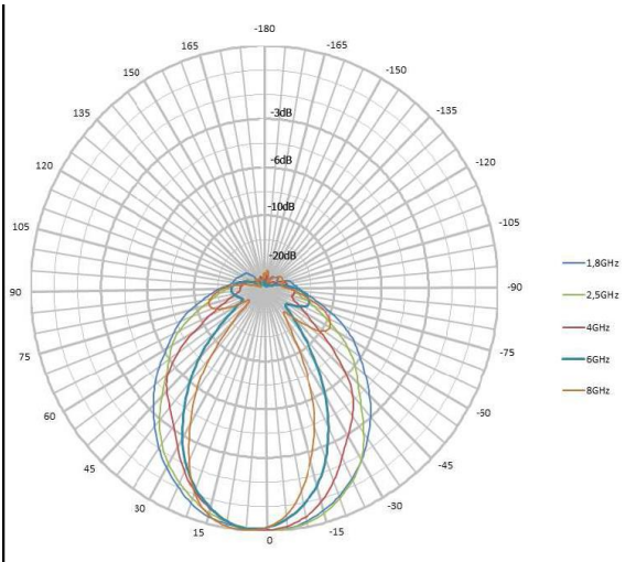
Vertical Pattern (typical) HyperLOG40x Series
