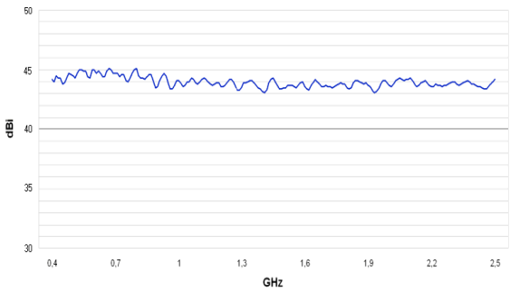
Gain Diagram HyperLOG 4025 X
