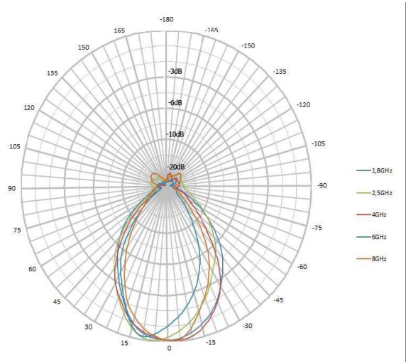
Horizontal Pattern (typical) HyperLOG 40x Series
