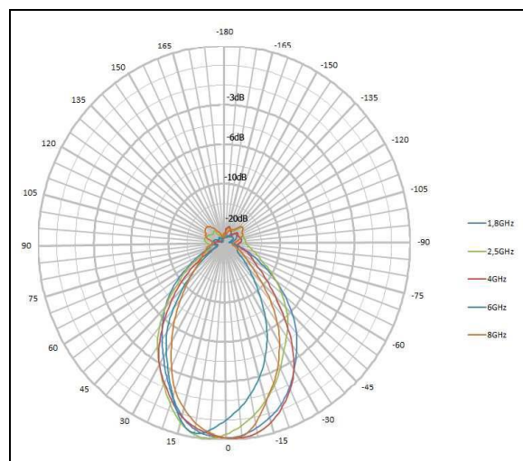
Vertical Pattern (typical) HyperLOG30x Series
