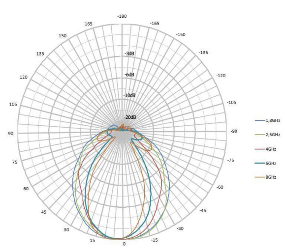
Horizontal Pattern (typical) HyperLOG 30x Series
