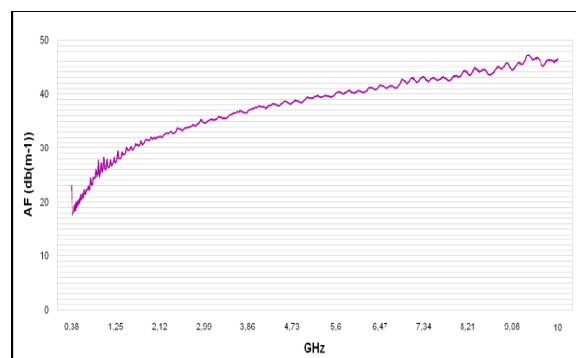
Antenna factor HyperLOG 30100X
