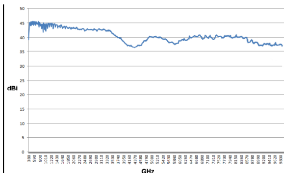
Gain Diagram HyperLOG30100X
