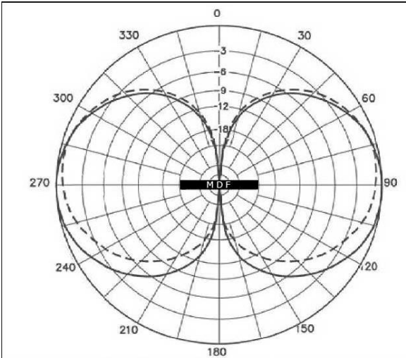
Antenna Pattern
