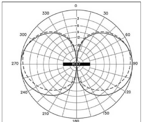
Antenna Pattern
