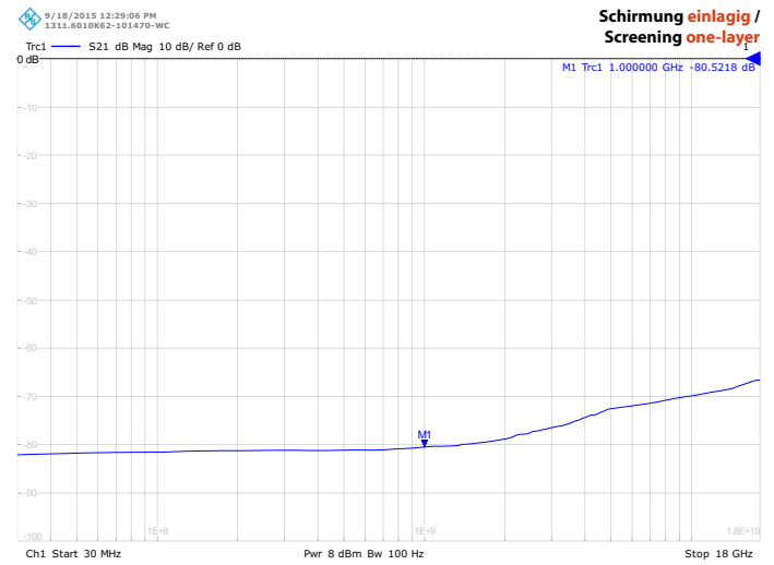
Schirmung zweilagig / Screening two-layer
