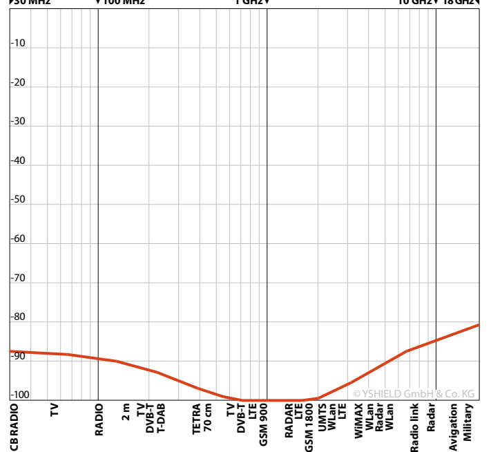
Shielding wallpaper YCF-100-100 Measurement to ASTM D4935-10
