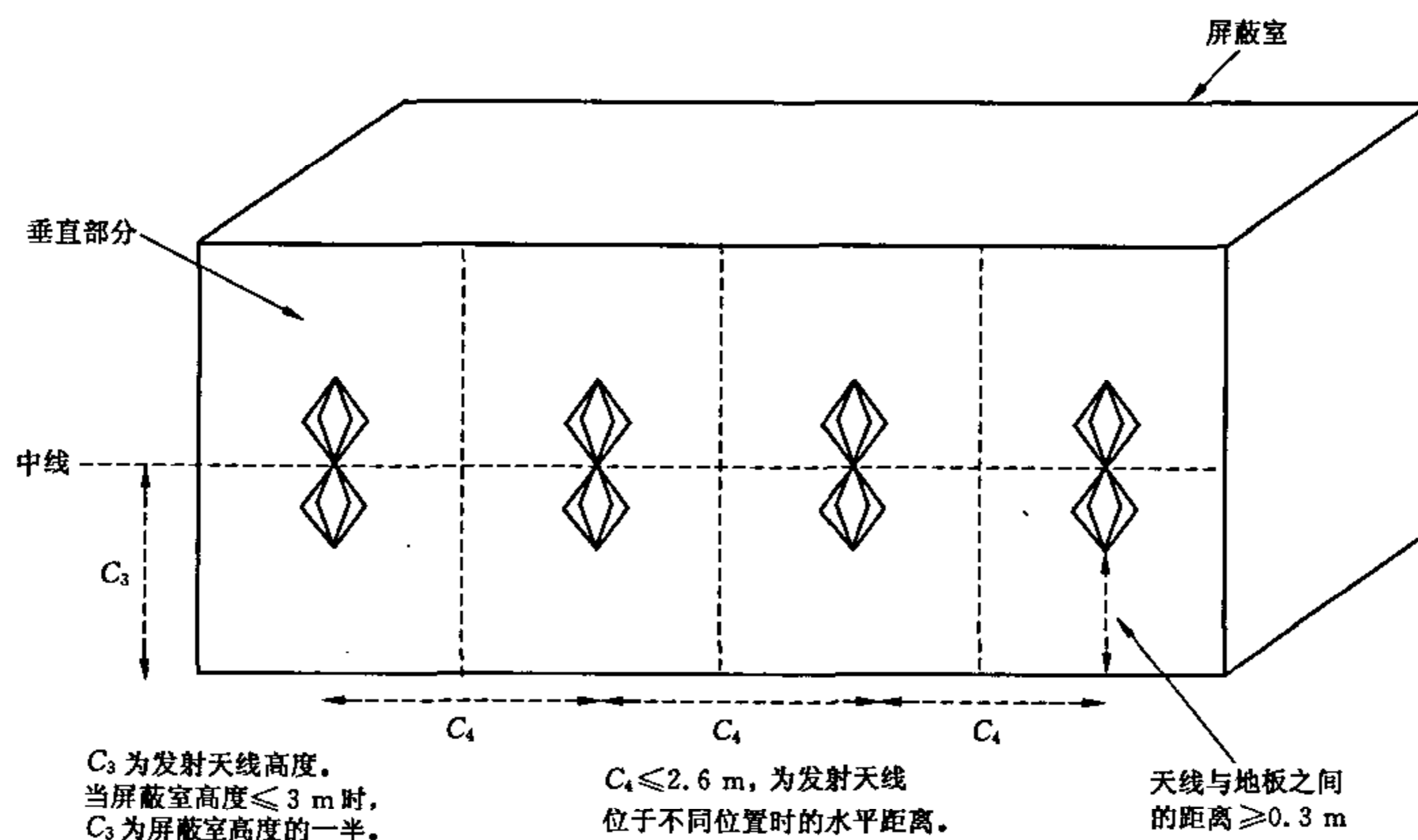
d) 谐振范围测量发射天线布置(垂直极化), 20 MHz~100 MHz
