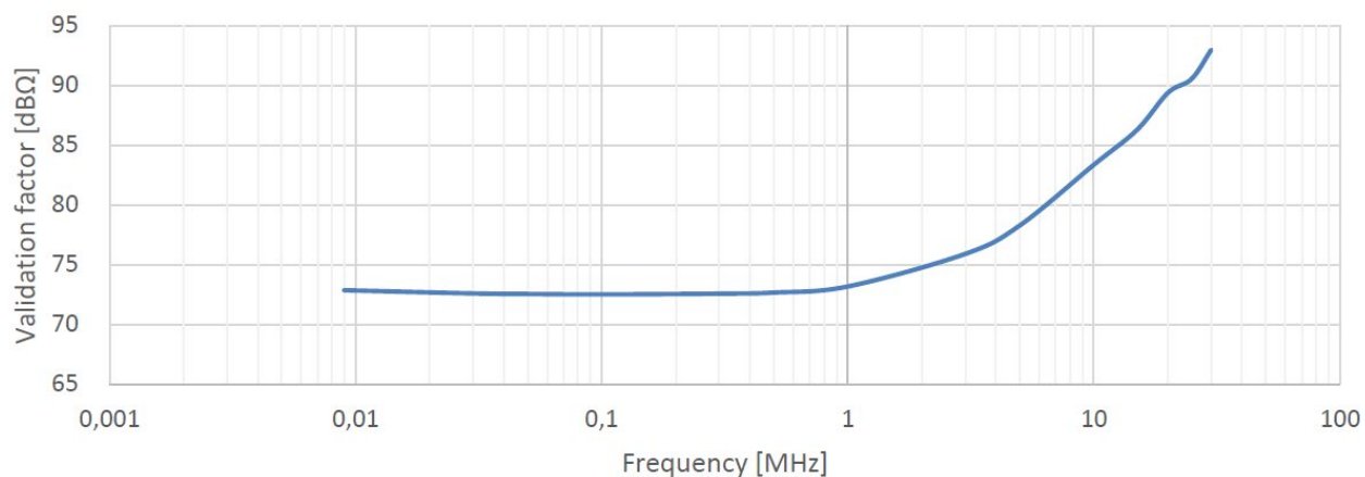
Measured Validation Factor
