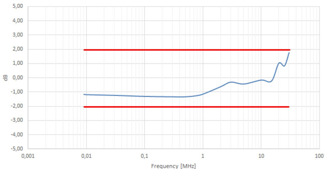
Antenna Correction Factor [dB]
